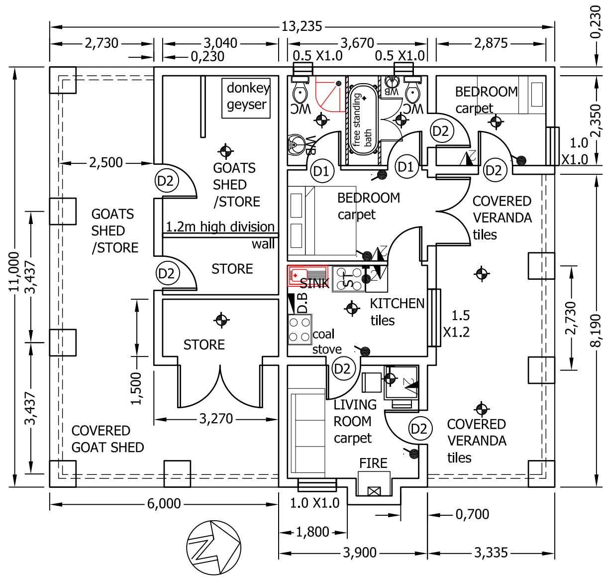
FLOOR PLAN
