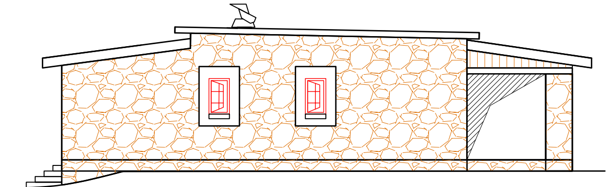
WEST ELEVATION
